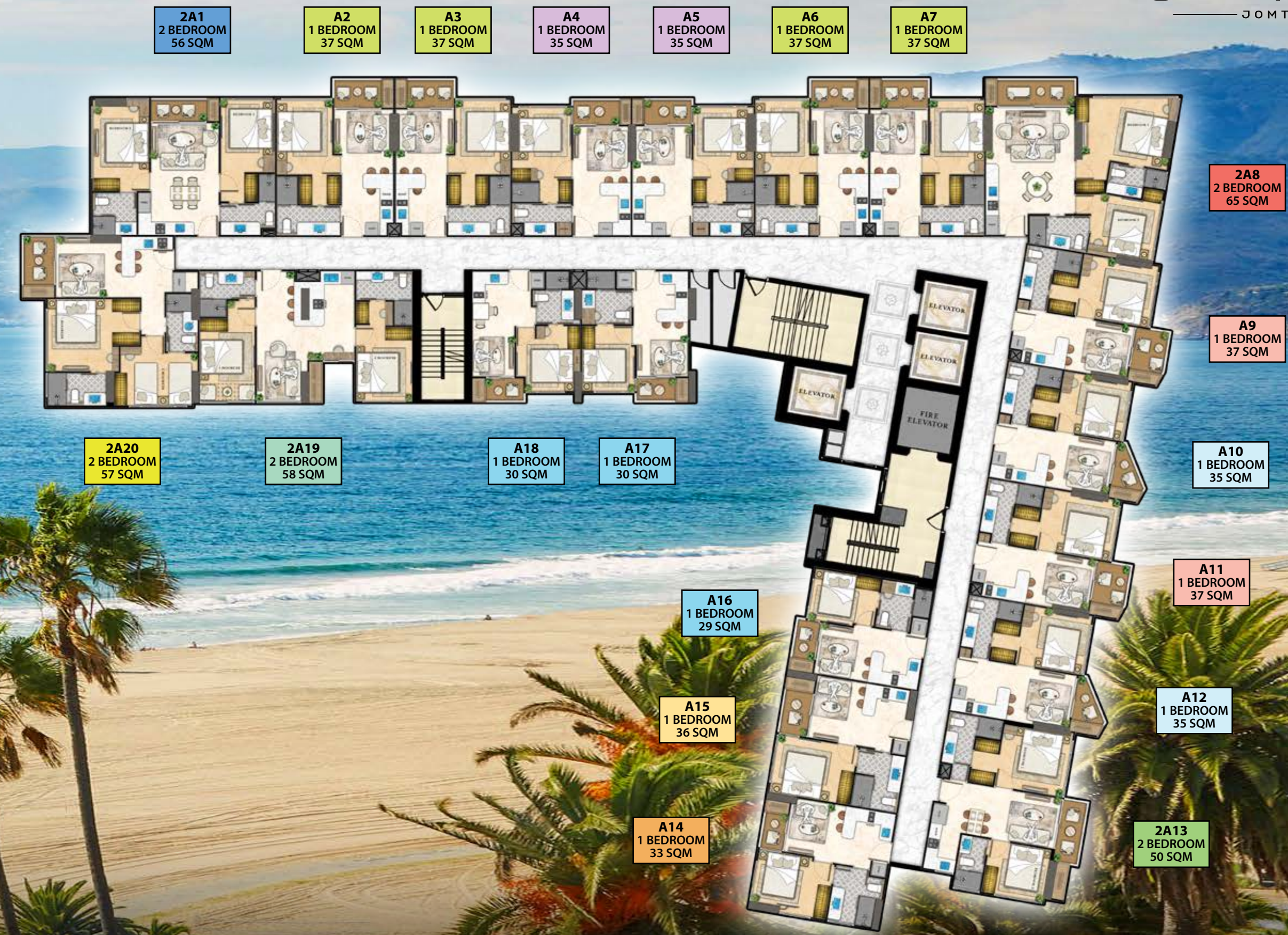
12th Floor Plan
